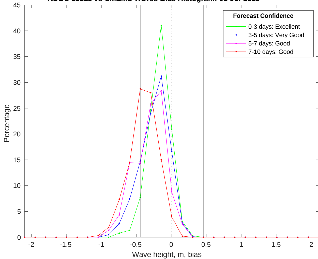
NDBC 52213 vs CMEMS Waves Bias Histogram: 01-Jul-2025
