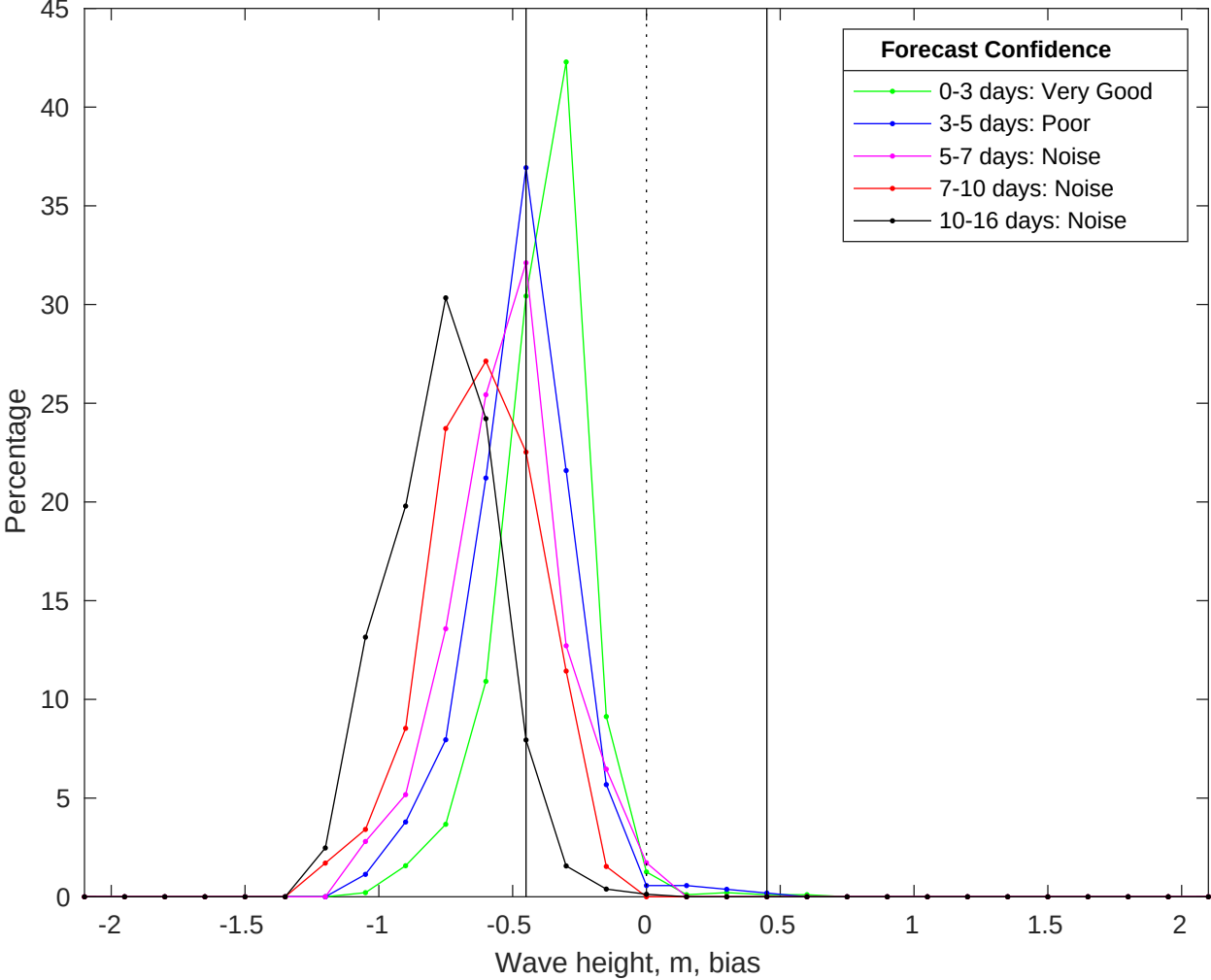
NDBC 52213 vs GFS Waves Bias Histogram: 01-Jul-2025
