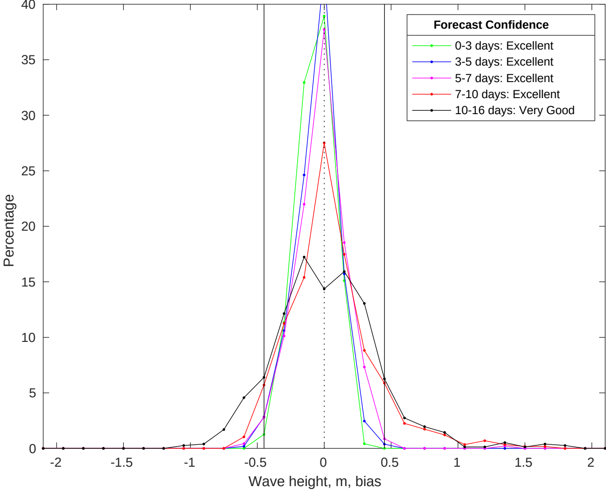
NDBC 41004 vs GFS Waves Bias Histogram: 02-Jul-2025
