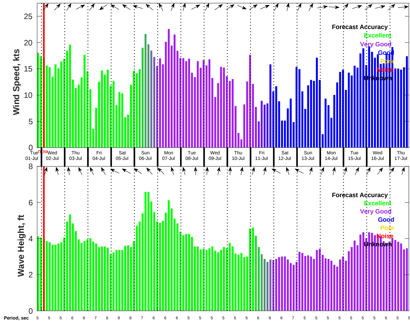
Wind & Wave Forecast for NDBC 41004 from 01-Jul-2025 19:00:00 to 17-Jul-2025 19:00:00
