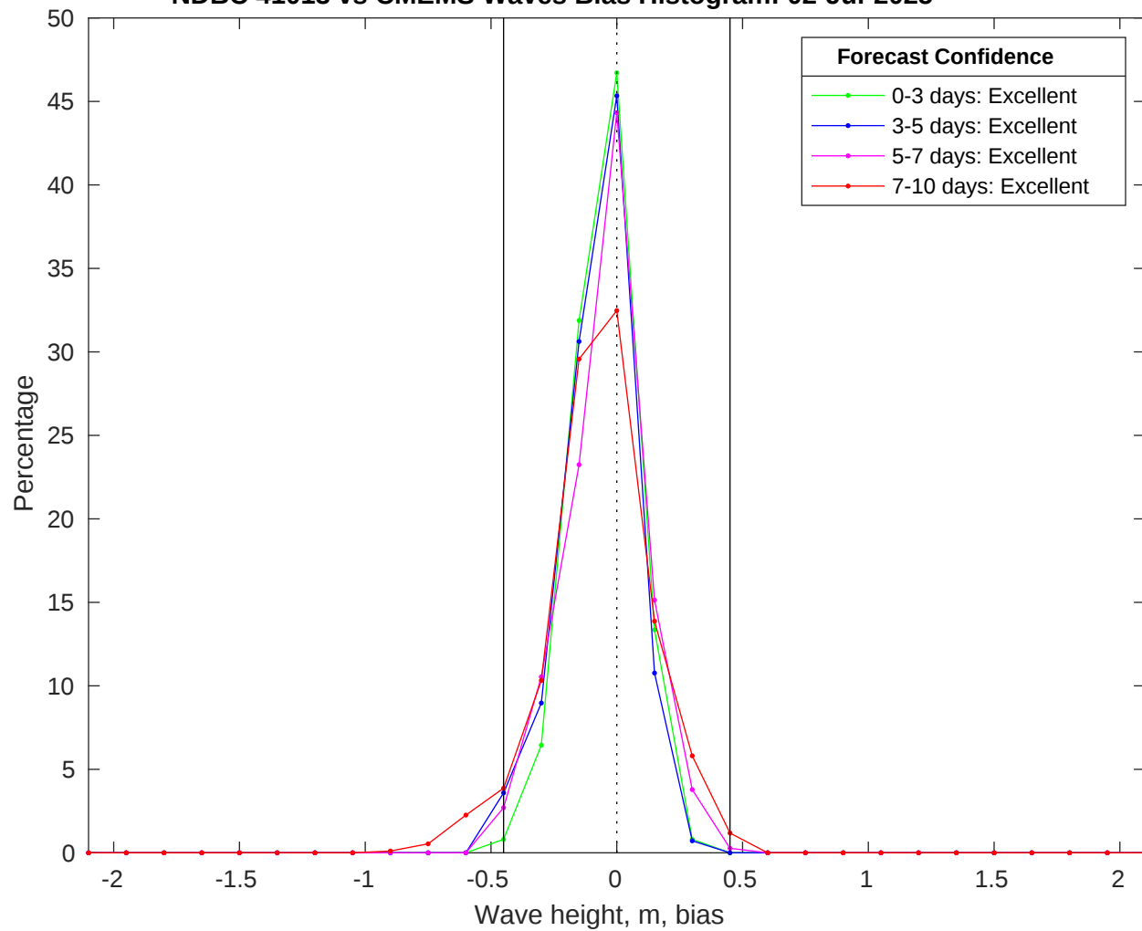
NDBC 41013 vs CMEMS Waves Bias Histogram: 02-Jul-2025
