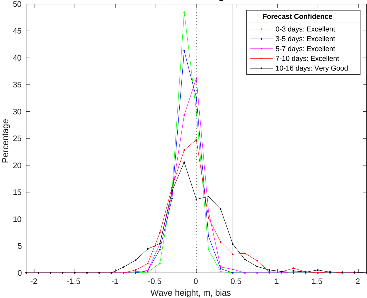
NDBC 41013 vs GFS Waves Bias Histogram: 02-Jul-2025
