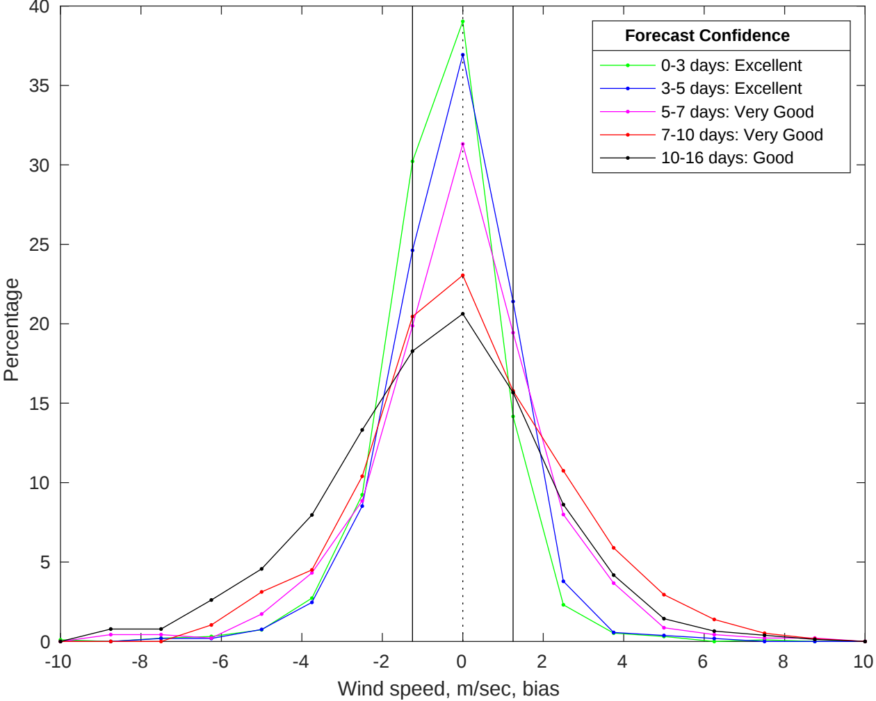
NDBC 41013 vs GFS Winds Bias Histogram: 02-Jul-2025
