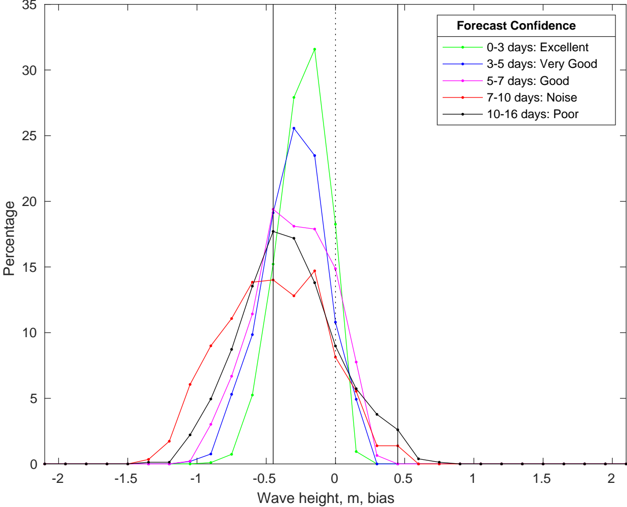
NDBC 41040 vs GFS Waves Bias Histogram: 02-Jul-2025
