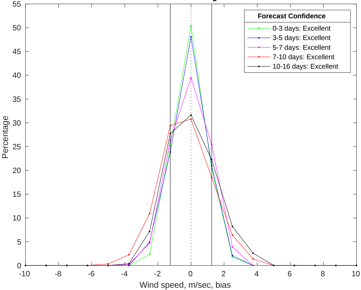
NDBC 41040 vs GFS Winds Bias Histogram: 02-Jul-2025
