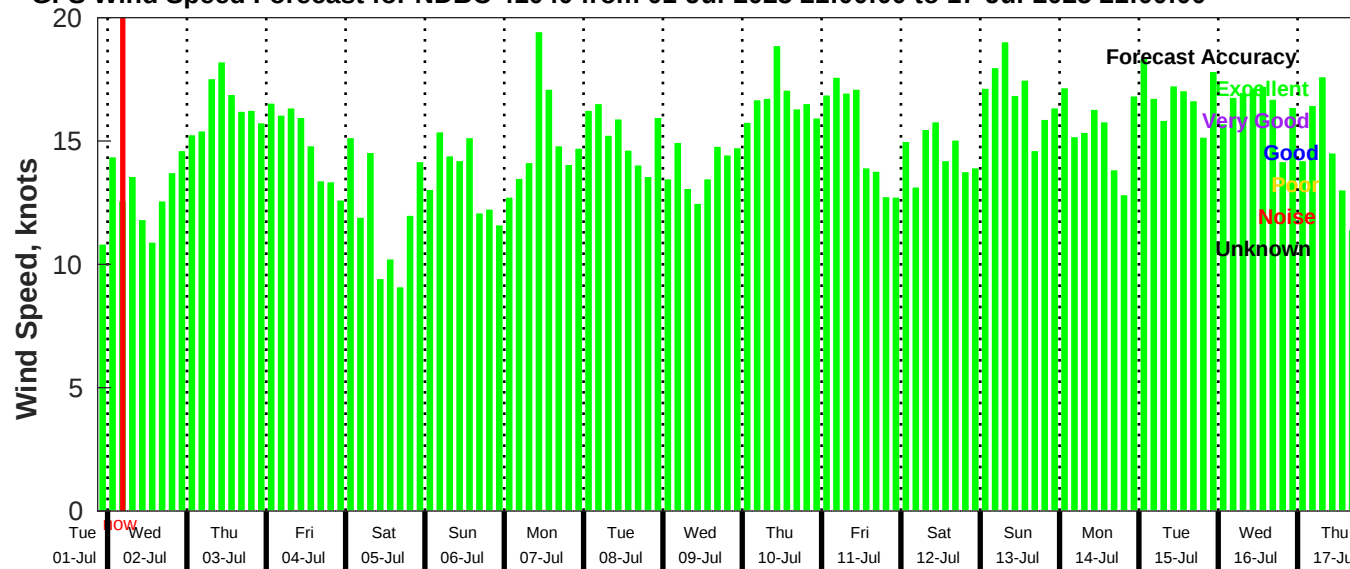
GFS Wind Speed Forecast for NDBC 41040 from 01-Jul-2025 21:00:00 to 17-Jul-2025 21:00:00
