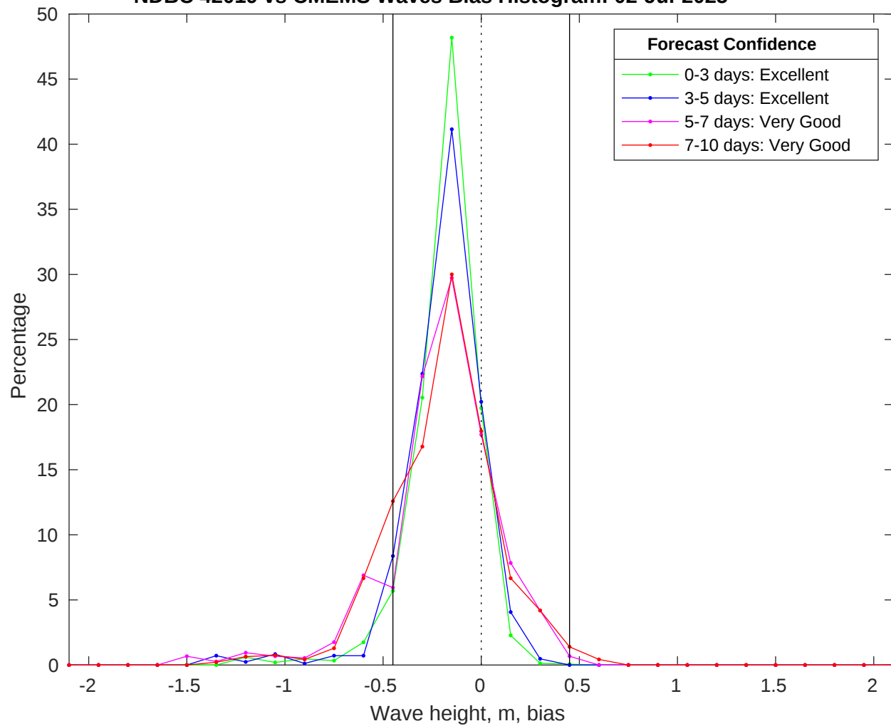
NDBC 42019 vs CMEMS Waves Bias Histogram: 02-Jul-2025
