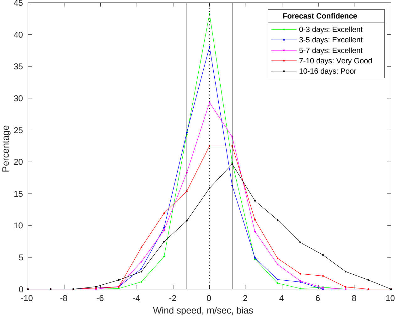
NDBC 42019 vs GFS Winds Bias Histogram: 02-Jul-2025
