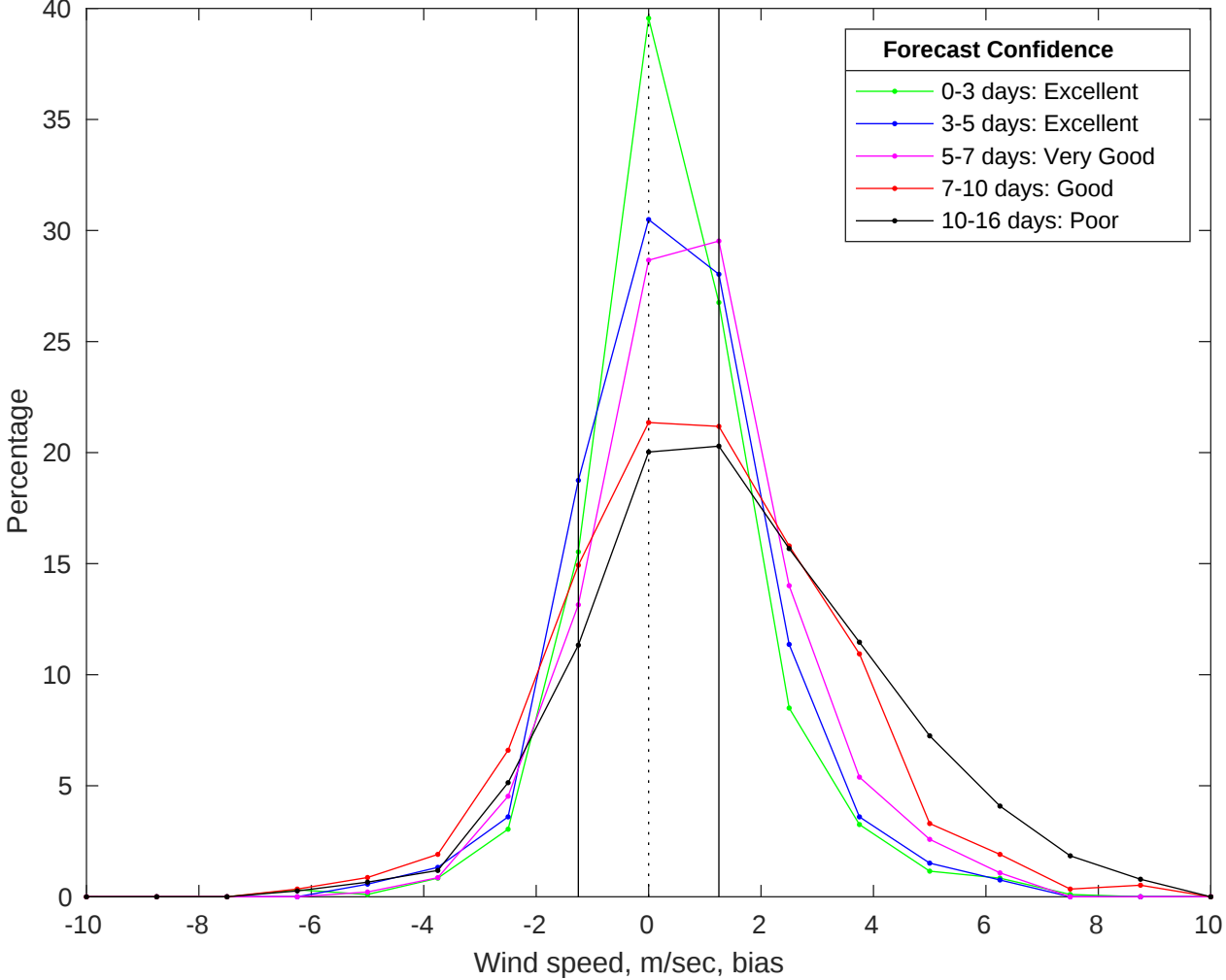
NDBC 42020 vs GFS Winds Bias Histogram: 02-Jul-2025
