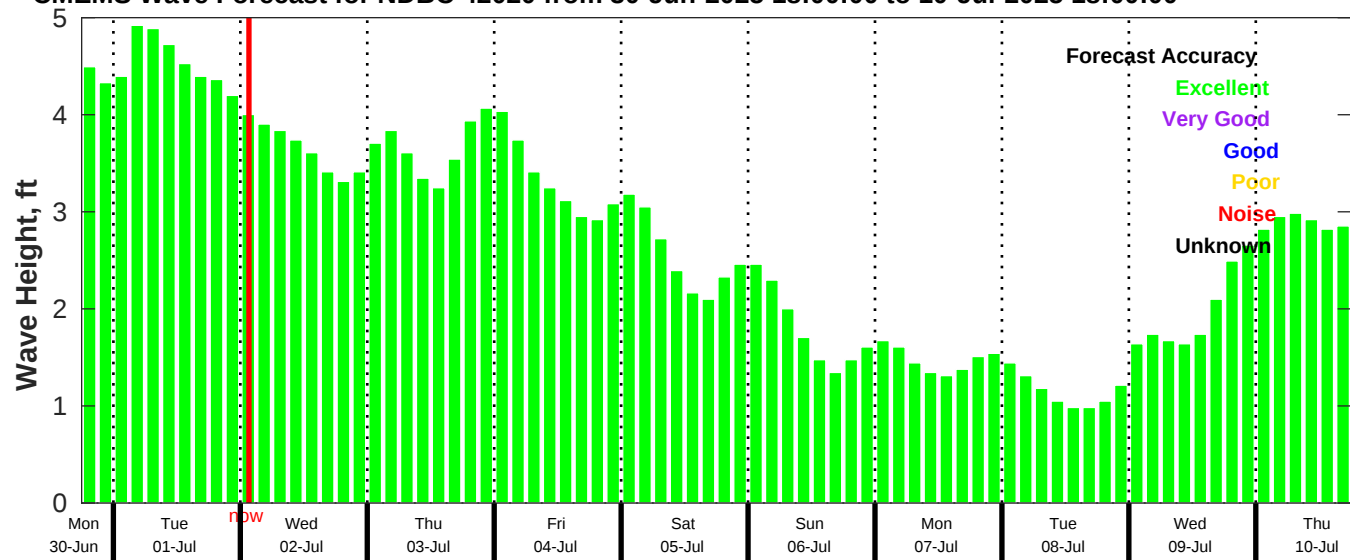
CMEMS Wave Forecast for NDBC 42020 from 30-Jun-2025 18:00:00 to 10-Jul-2025 18:00:00
