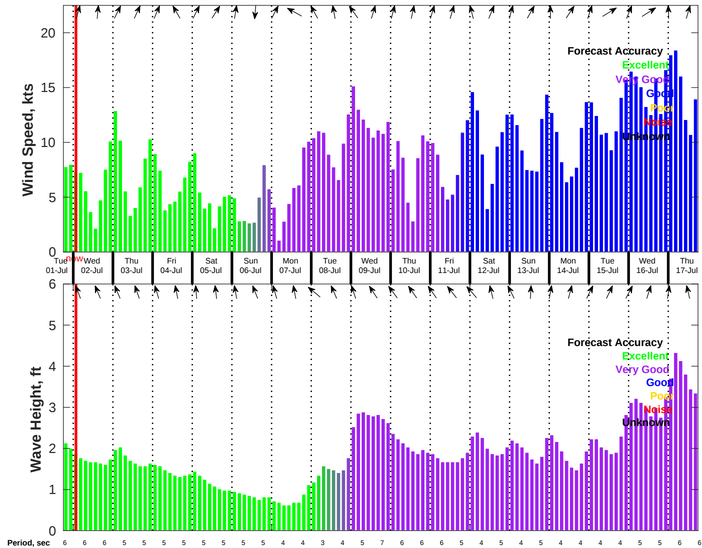
Wind & Wave Forecast for NDBC 42035 from 01-Jul-2025 18:00:00 to 17-Jul-2025 18:00:00
