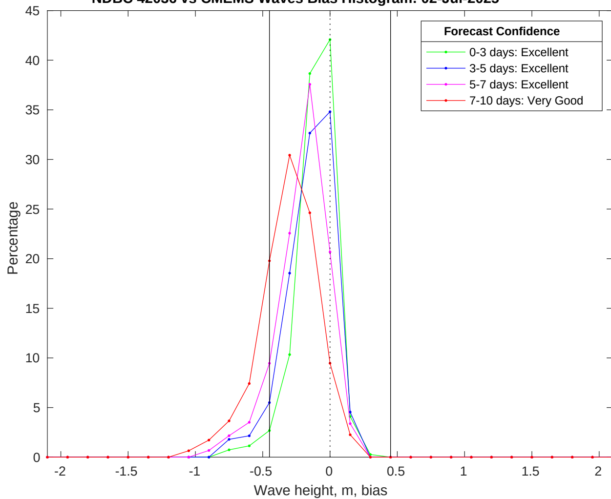
NDBC 42036 vs CMEMS Waves Bias Histogram: 02-Jul-2025
