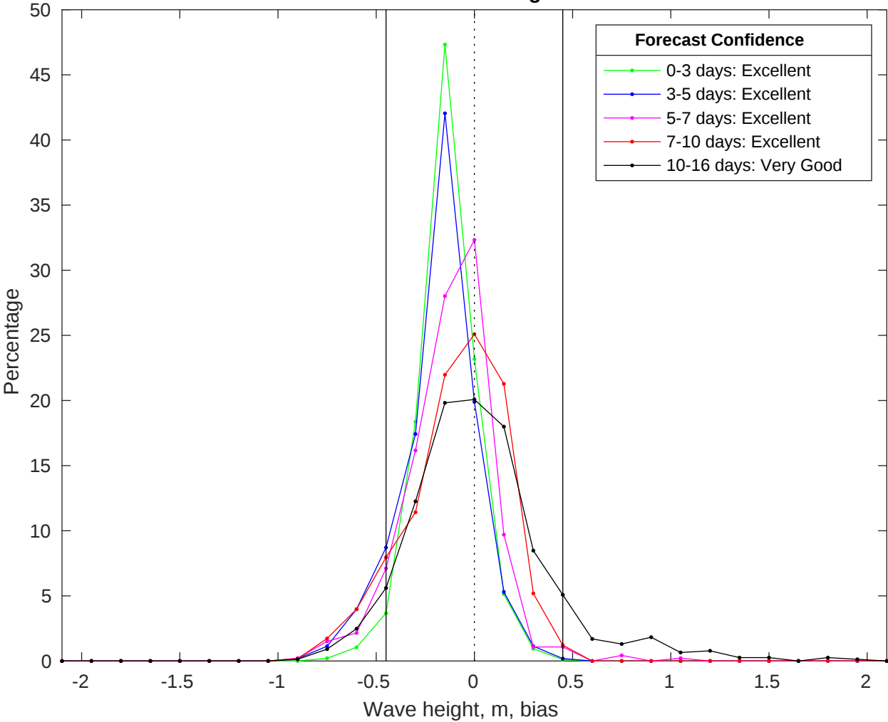
NDBC 42036 vs GFS Waves Bias Histogram: 02-Jul-2025
