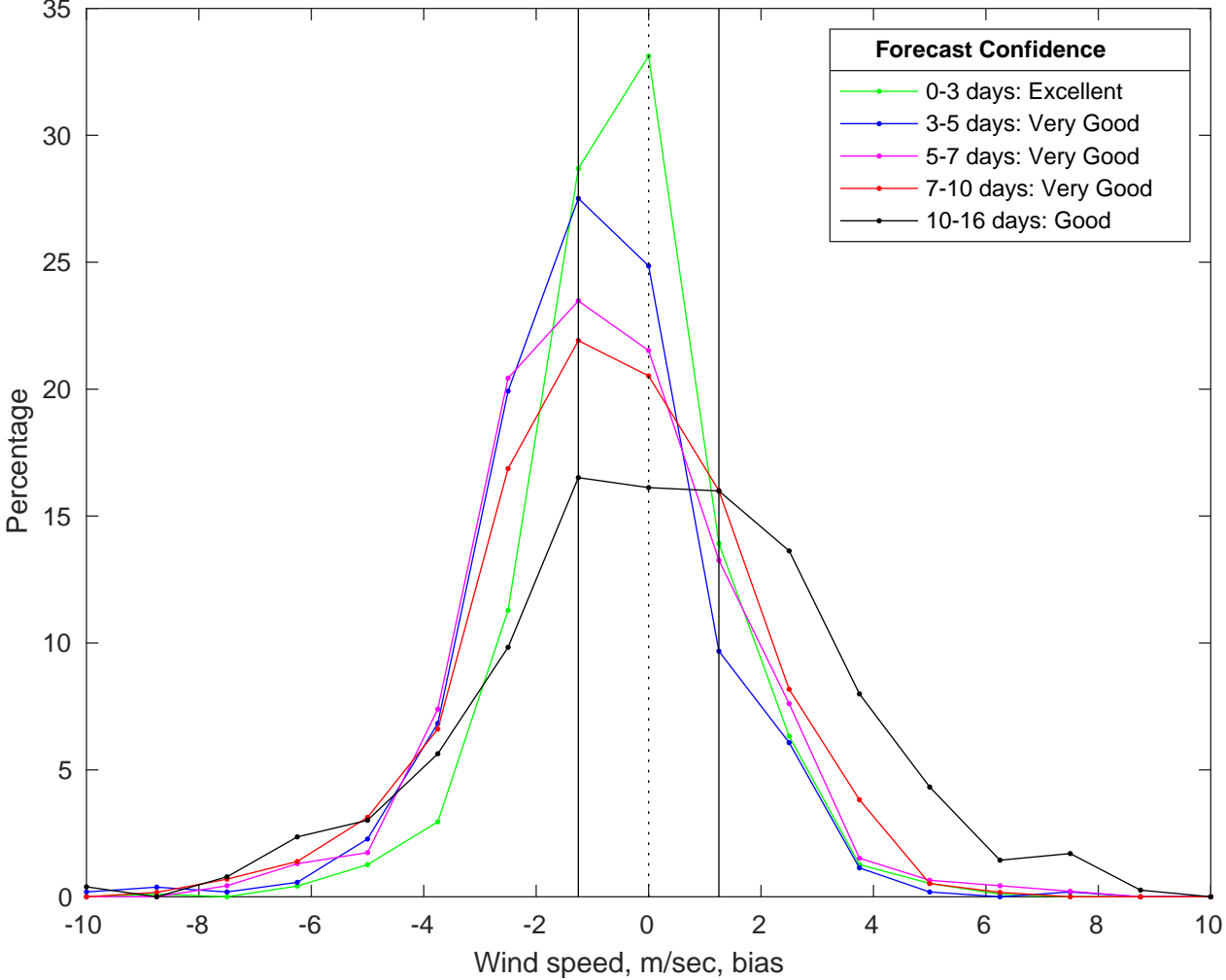
NDBC 42036 vs GFS Winds Bias Histogram: 02-Jul-2025
