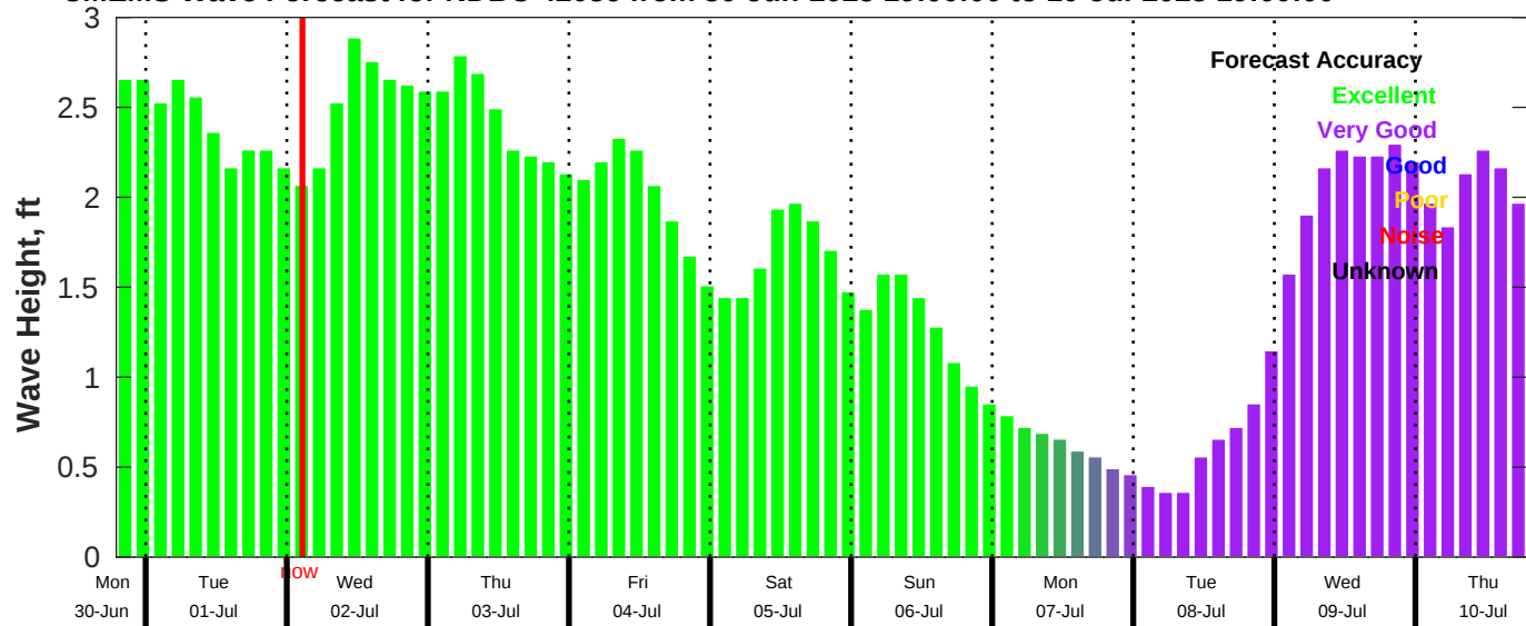
CMEMS Wave Forecast for NDBC 42036 from 30-Jun-2025 19:00:00 to 10-Jul-2025 19:00:00
