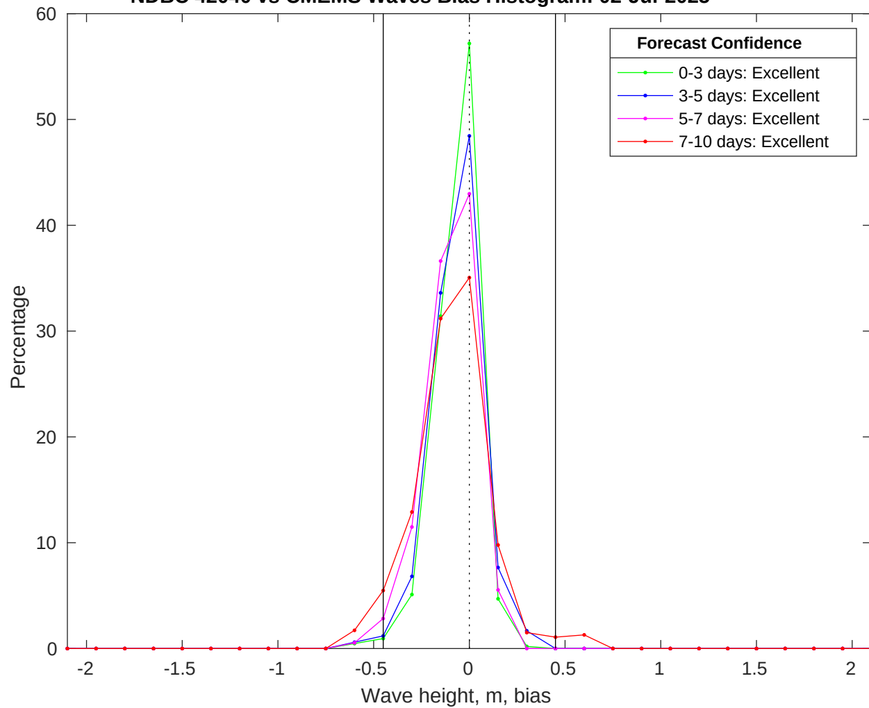
NDBC 42040 vs CMEMS Waves Bias Histogram: 02-Jul-2025
