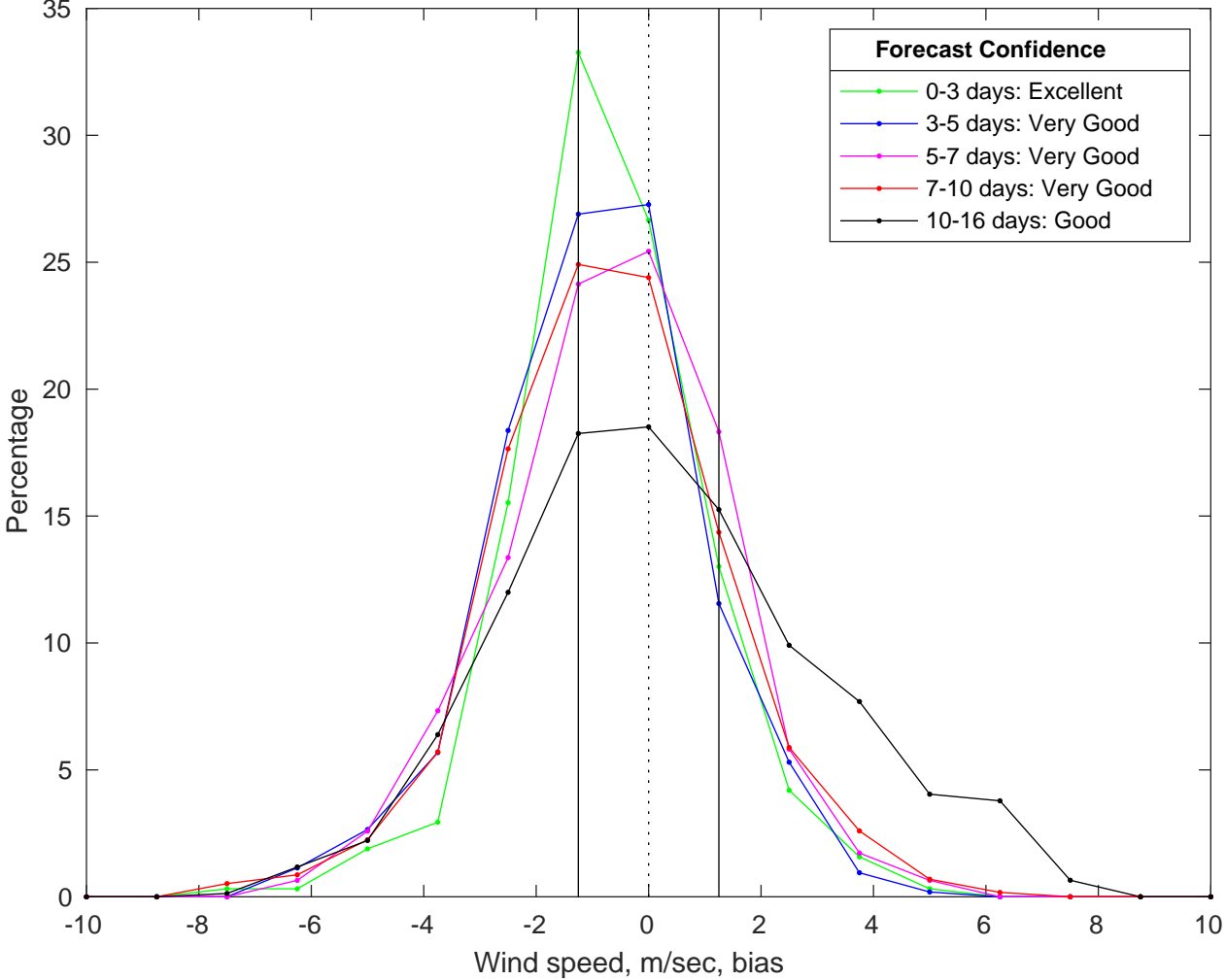
NDBC 42040 vs GFS Winds Bias Histogram: 02-Jul-2025
