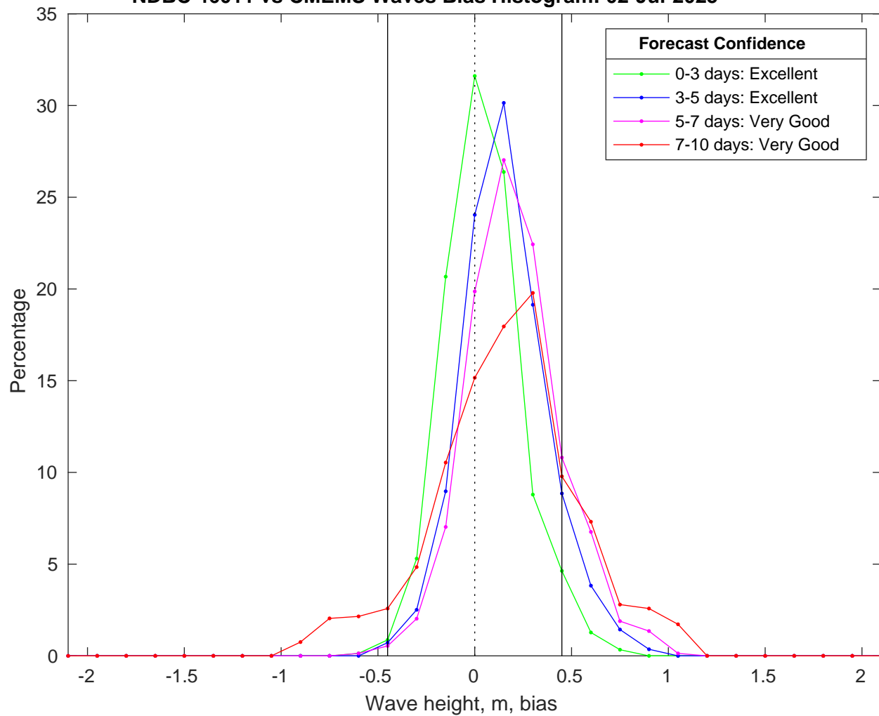
NDBC 46011 vs CMEMS Waves Bias Histogram: 02-Jul-2025
