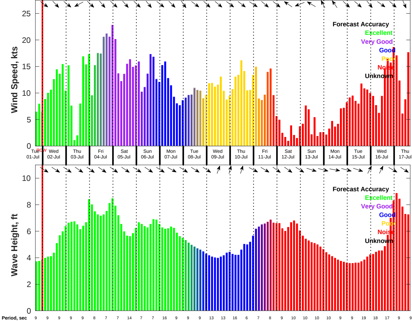
Wind & Wave Forecast for NDBC 46011 from 01-Jul-2025 16:00:00 to 17-Jul-2025 16:00:00
