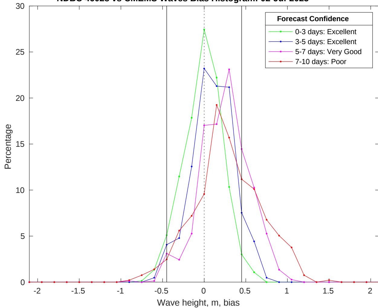
NDBC 46028 vs CMEMS Waves Bias Histogram: 02-Jul-2025
