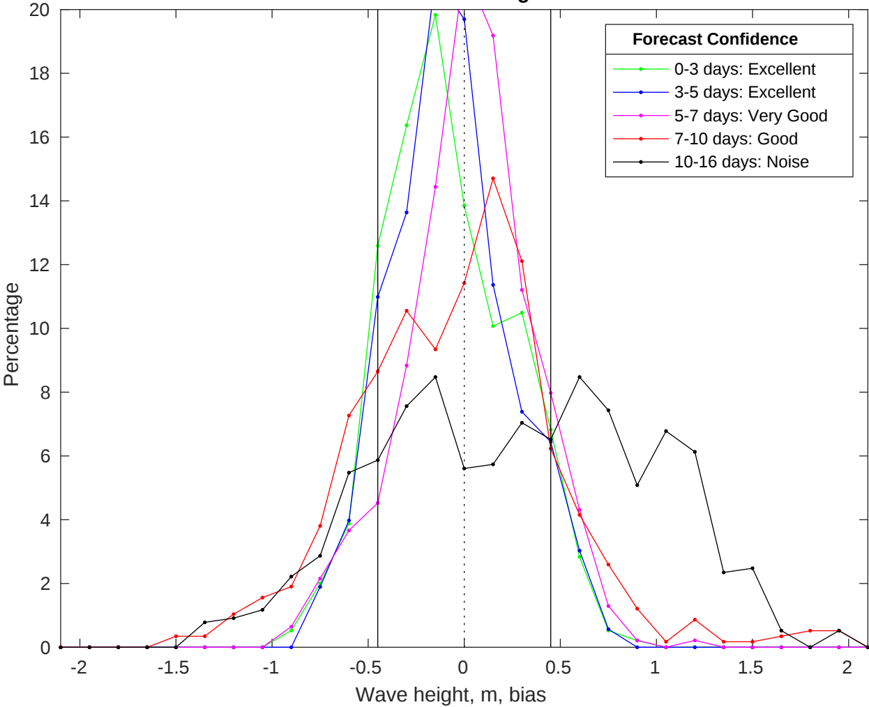
NDBC 46028 vs GFS Waves Bias Histogram: 02-Jul-2025
