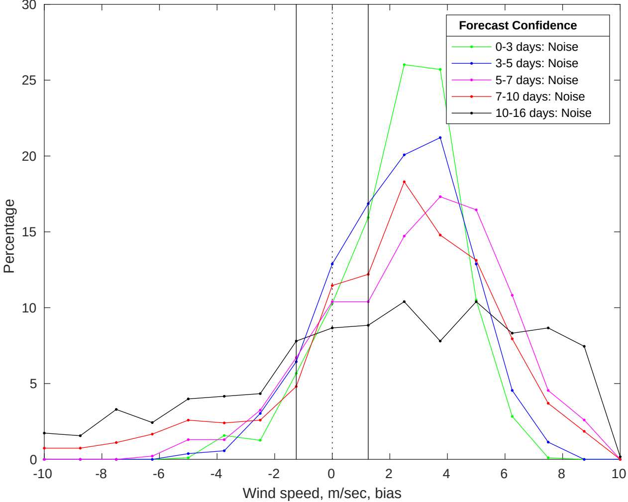
NDBC 46028 vs GFS Winds Bias Histogram: 02-Jul-2025
