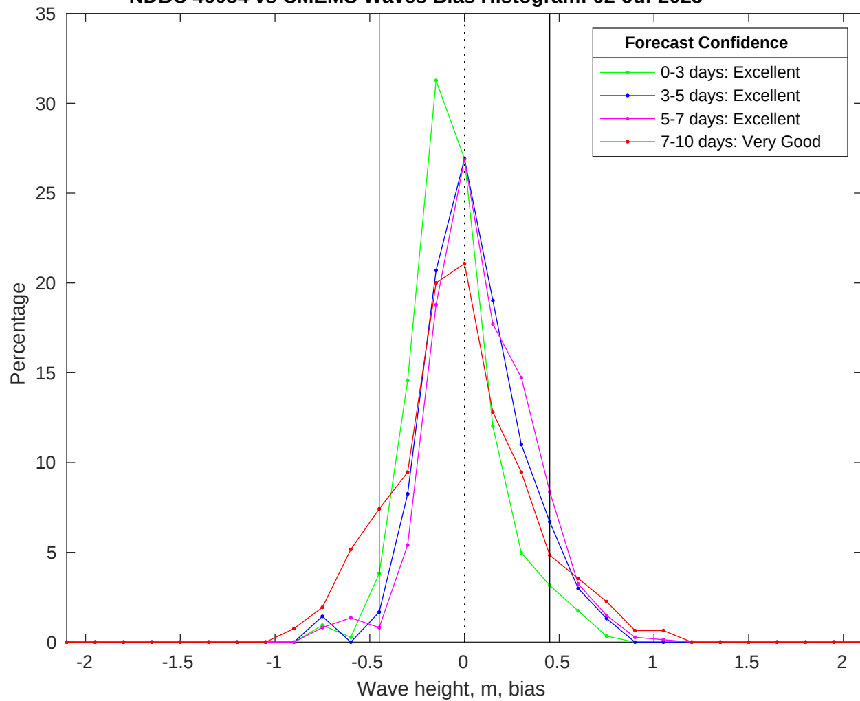
NDBC 46054 vs CMEMS Waves Bias Histogram: 02-Jul-2025
