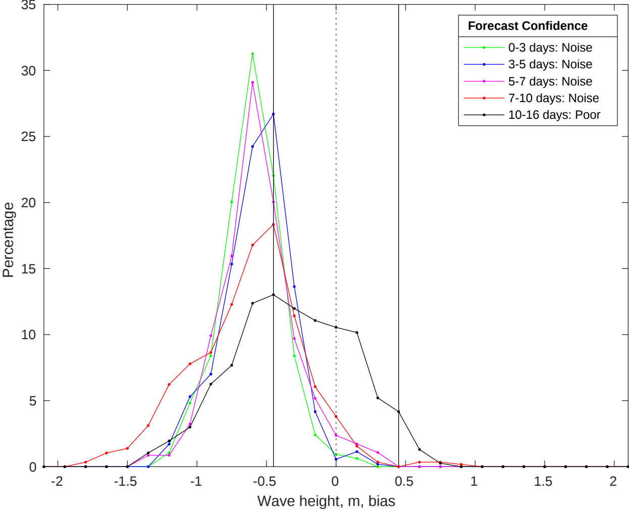
NDBC 46054 vs GFS Waves Bias Histogram: 02-Jul-2025
