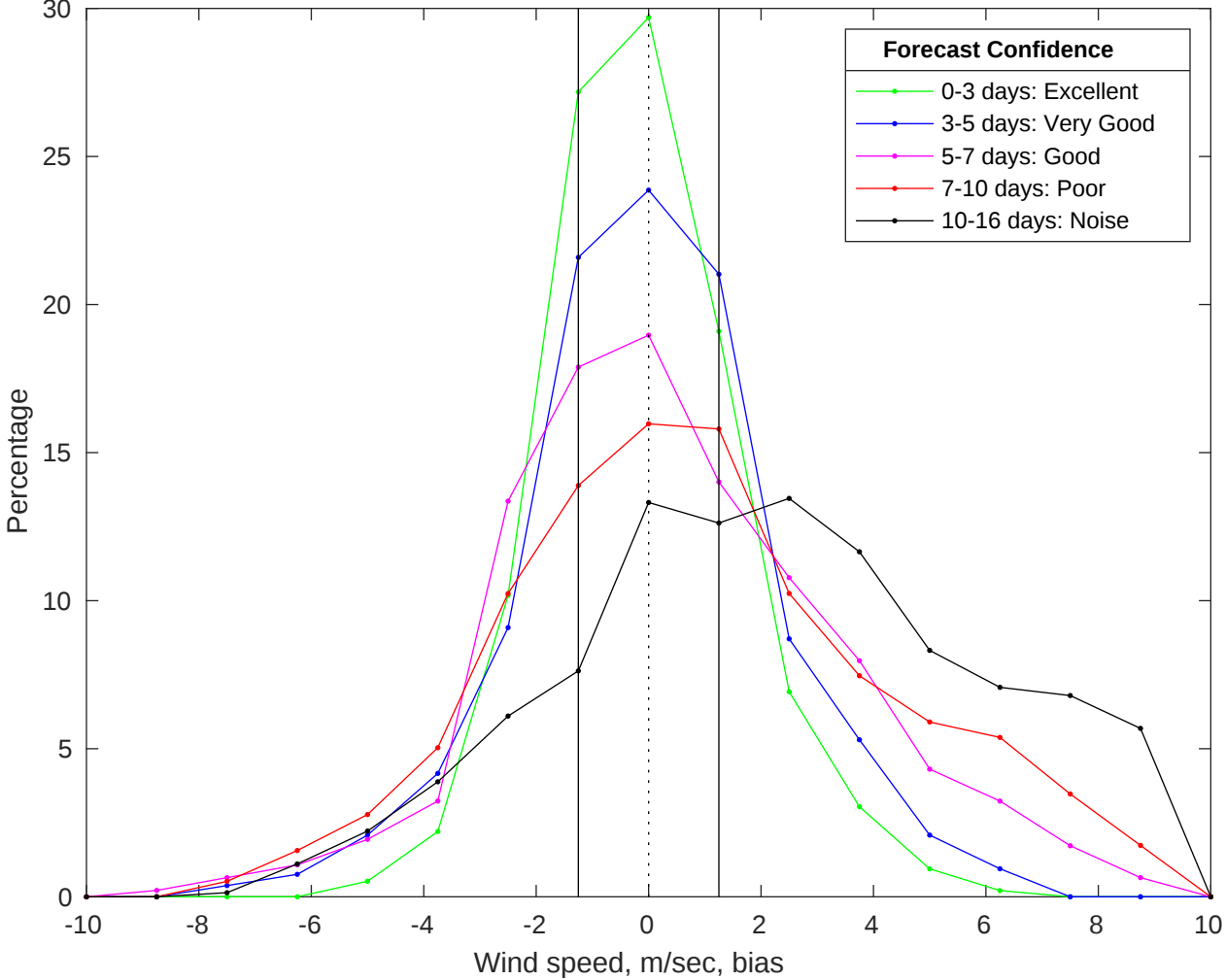
NDBC 46054 vs GFS Winds Bias Histogram: 02-Jul-2025
