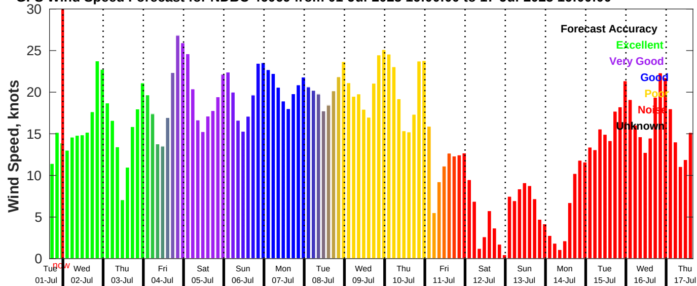
GFS Wind Speed Forecast for NDBC 46069 from 01-Jul-2025 16:00:00 to 17-Jul-2025 16:00:00
