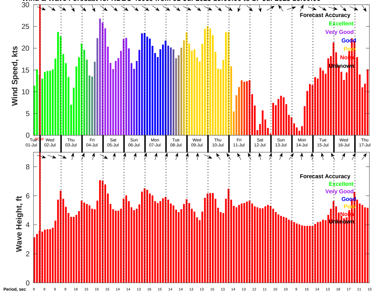
Wind & Wave Forecast for NDBC 46069 from 01-Jul-2025 16:00:00 to 17-Jul-2025 16:00:00
