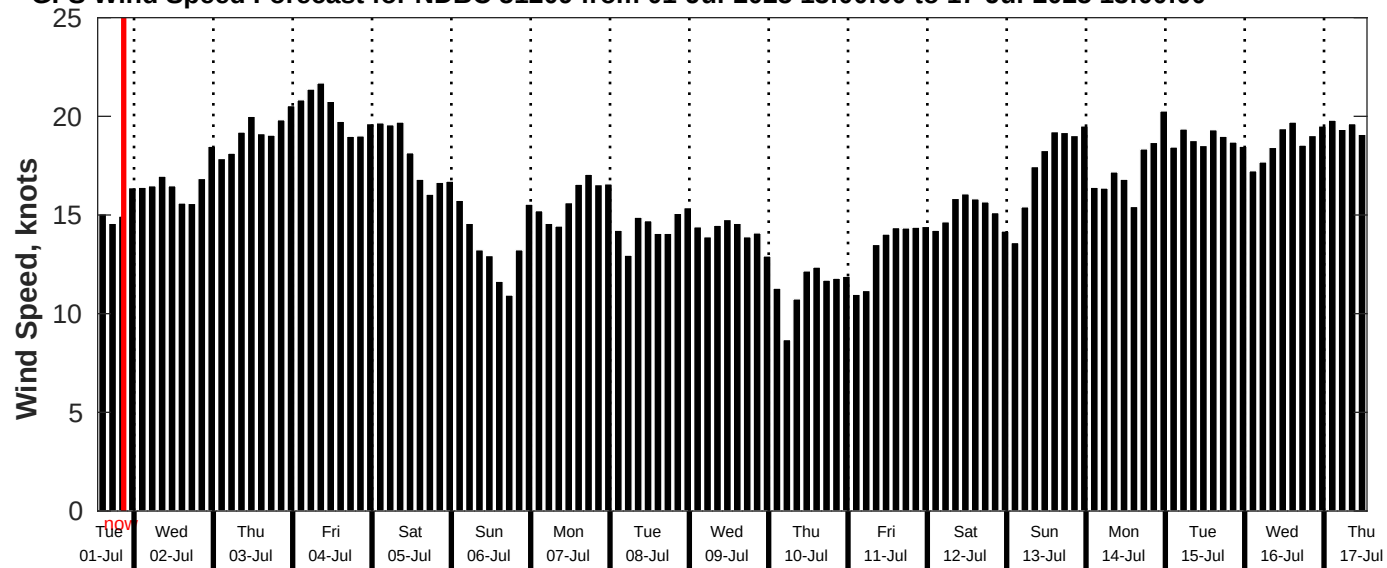
GFS Wind Speed Forecast for NDBC 51209 from 01-Jul-2025 13:00:00 to 17-Jul-2025 13:00:00
