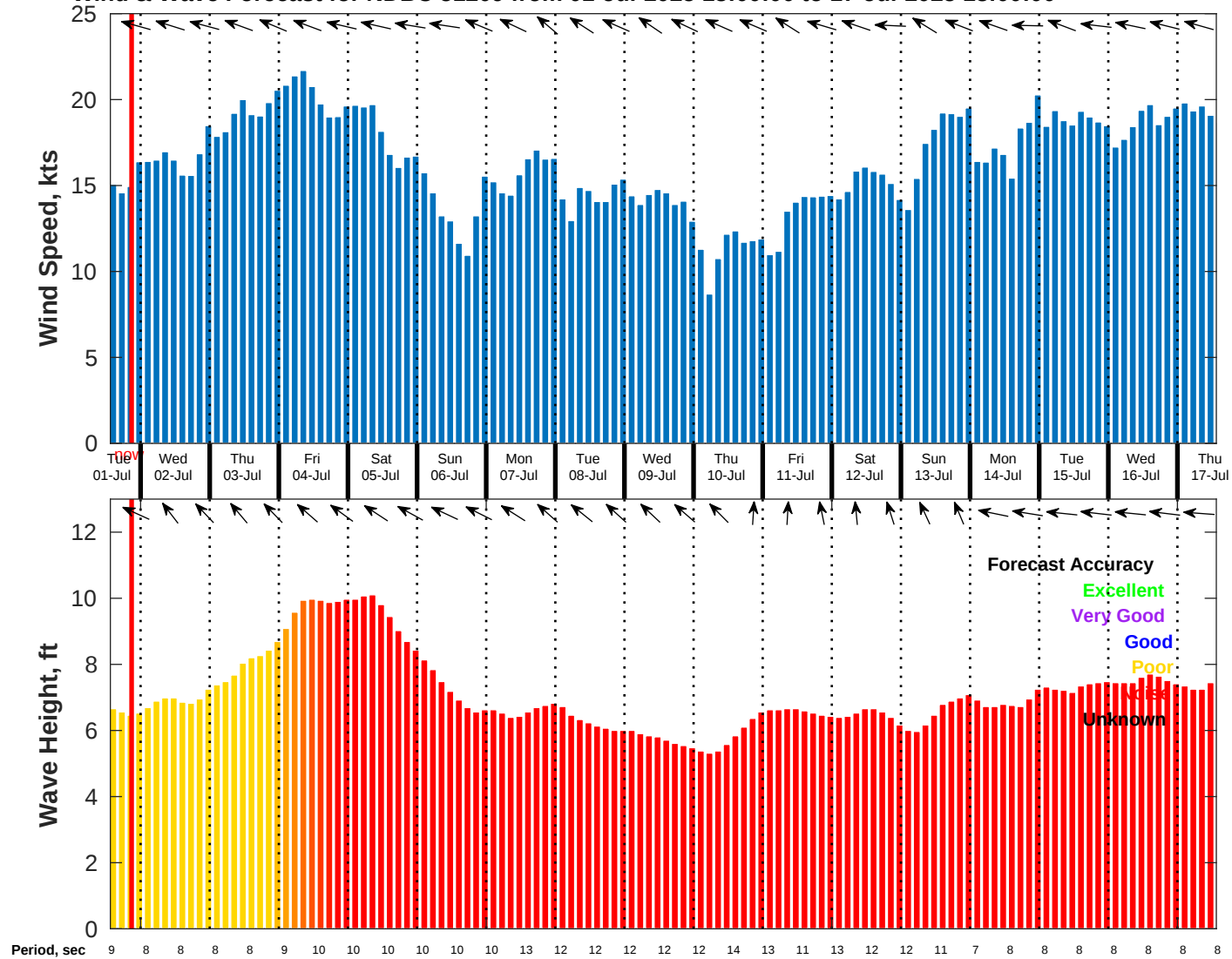
Wind & Wave Forecast for NDBC 51209 from 01-Jul-2025 13:00:00 to 17-Jul-2025 13:00:00
