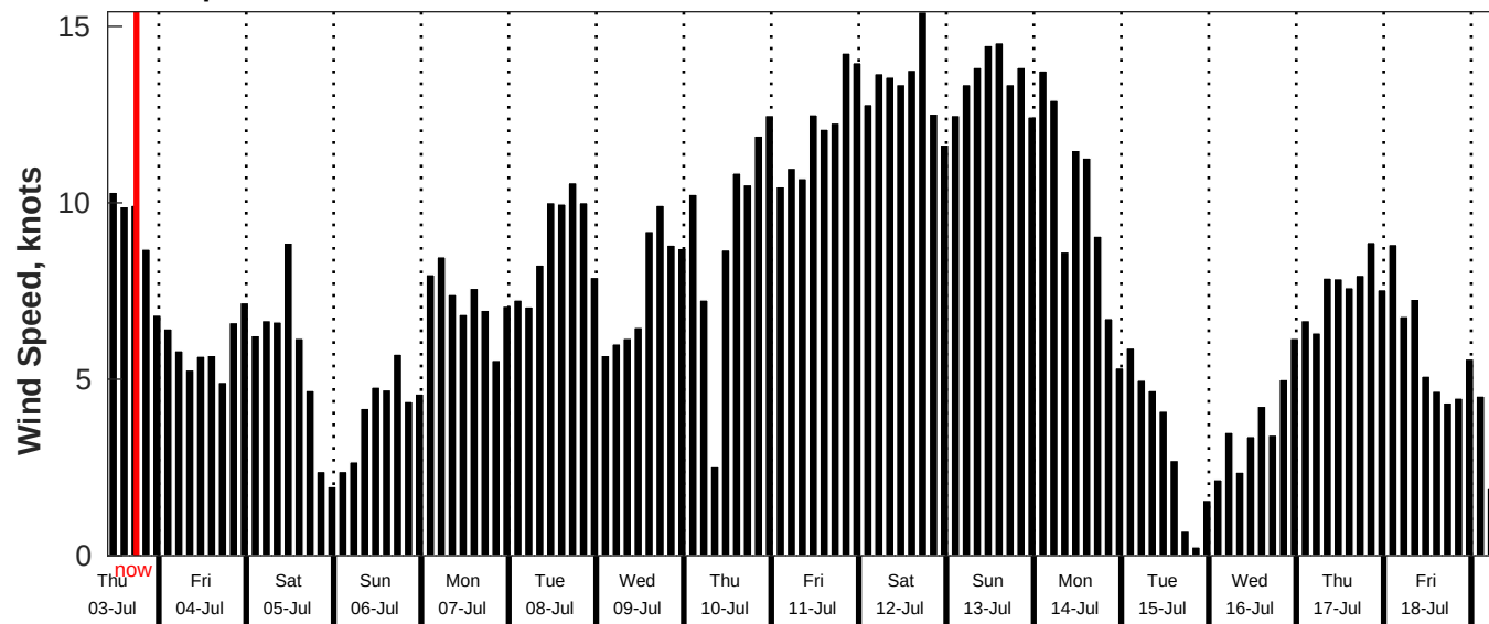
GFS Wind Speed Forecast for NDBC 52211 from 02-Jul-2025 10:00:00 to 18-Jul-2025 10:00:00
