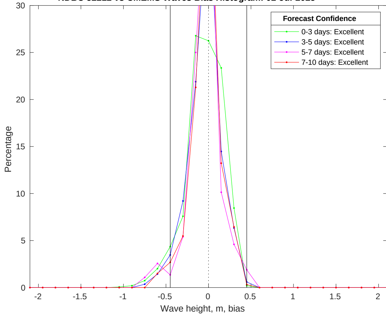
NDBC 52212 vs CMEMS Waves Bias Histogram: 02-Jul-2025
