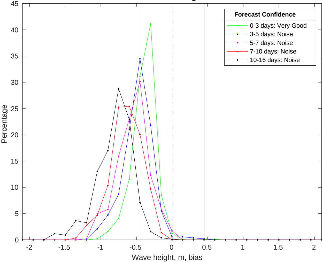
NDBC 52213 vs GFS Waves Bias Histogram: 02-Jul-2025
