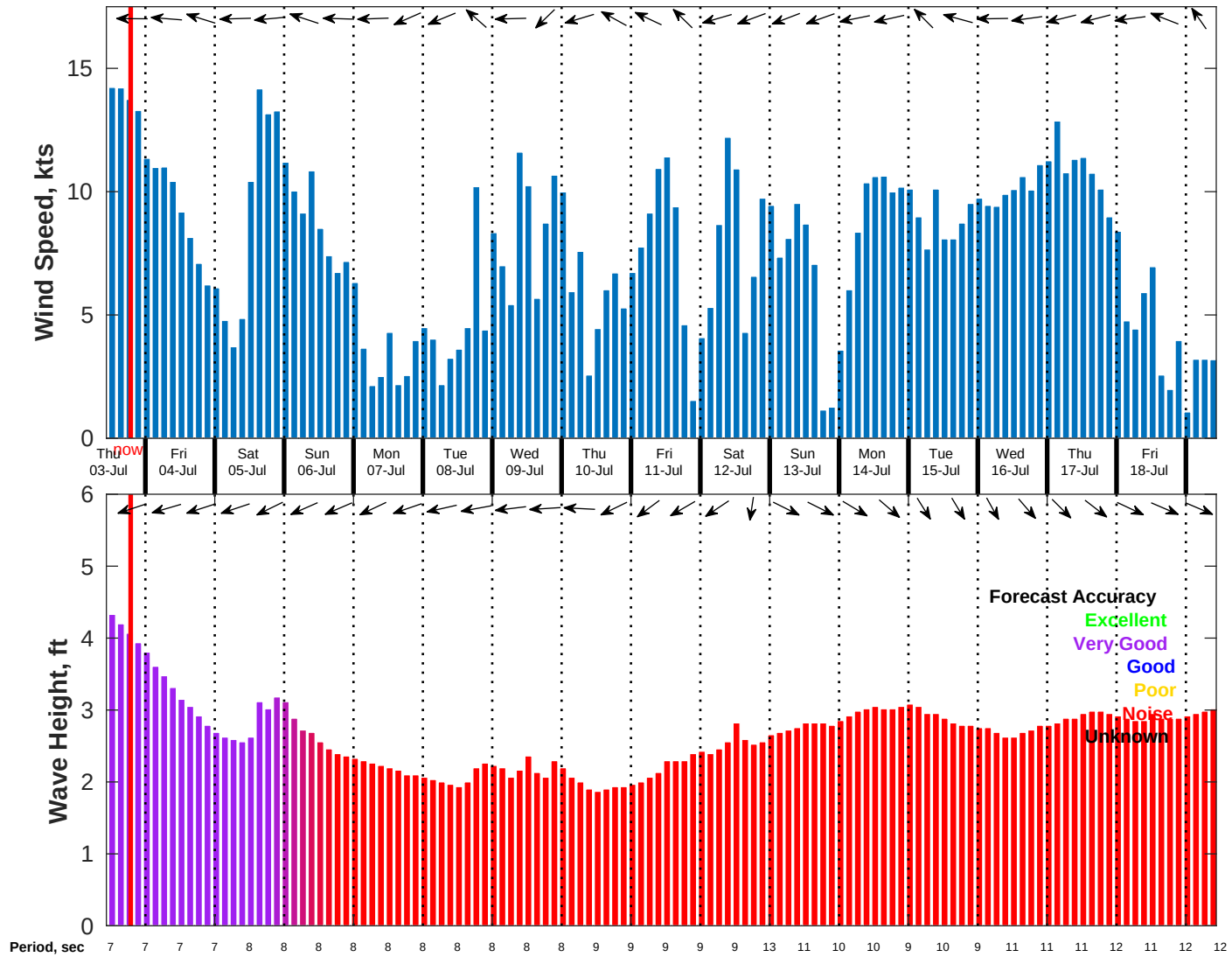
Wind & Wave Forecast for NDBC 52213 from 02-Jul-2025 11:00:00 to 18-Jul-2025 11:00:00
