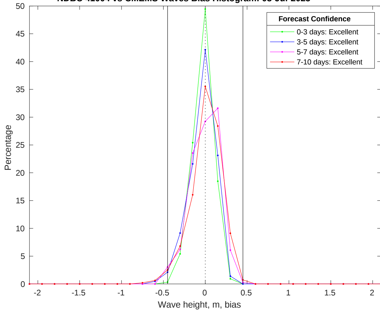
NDBC 41004 vs CMEMS Waves Bias Histogram: 03-Jul-2025
