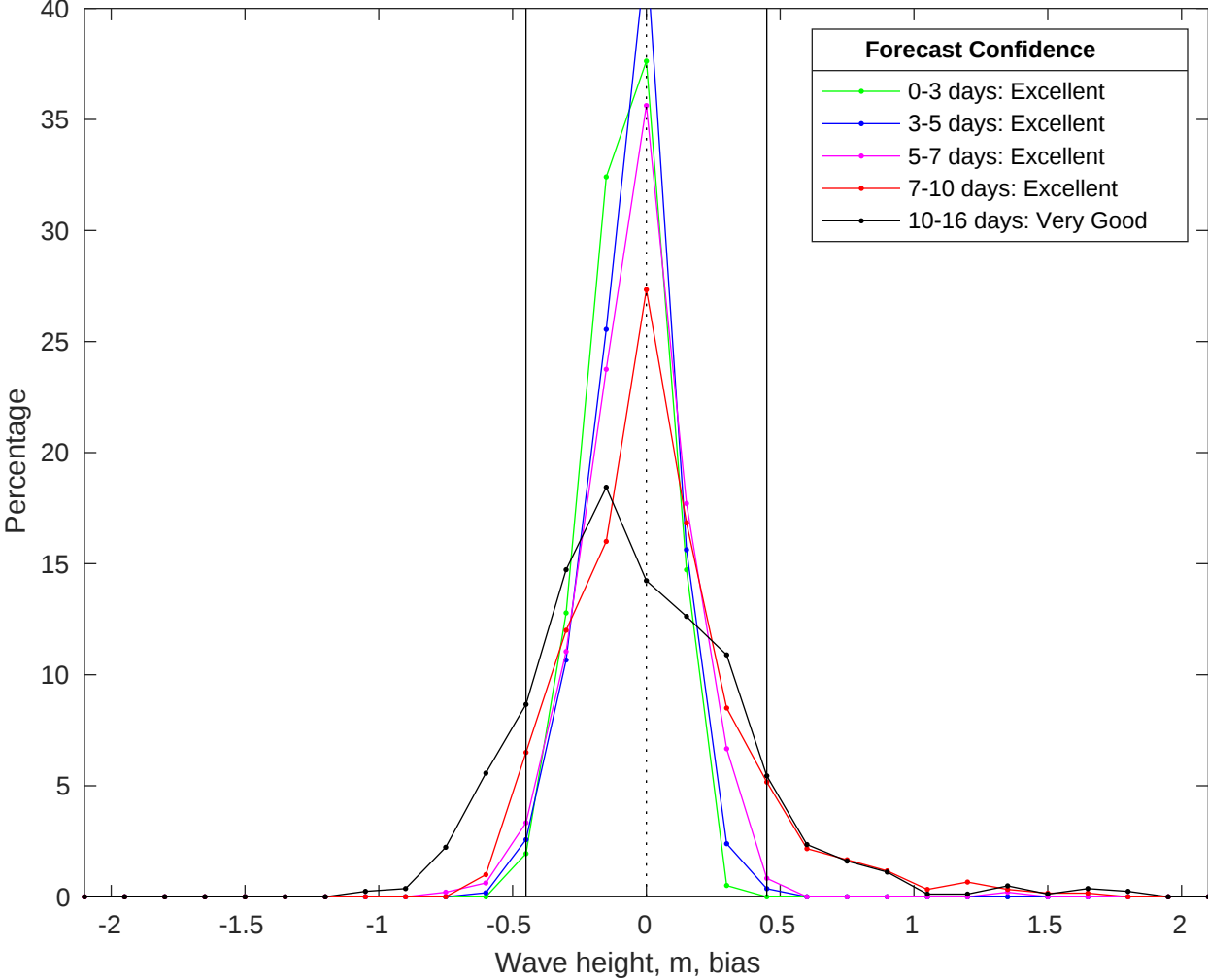
NDBC 41004 vs GFS Waves Bias Histogram: 03-Jul-2025
