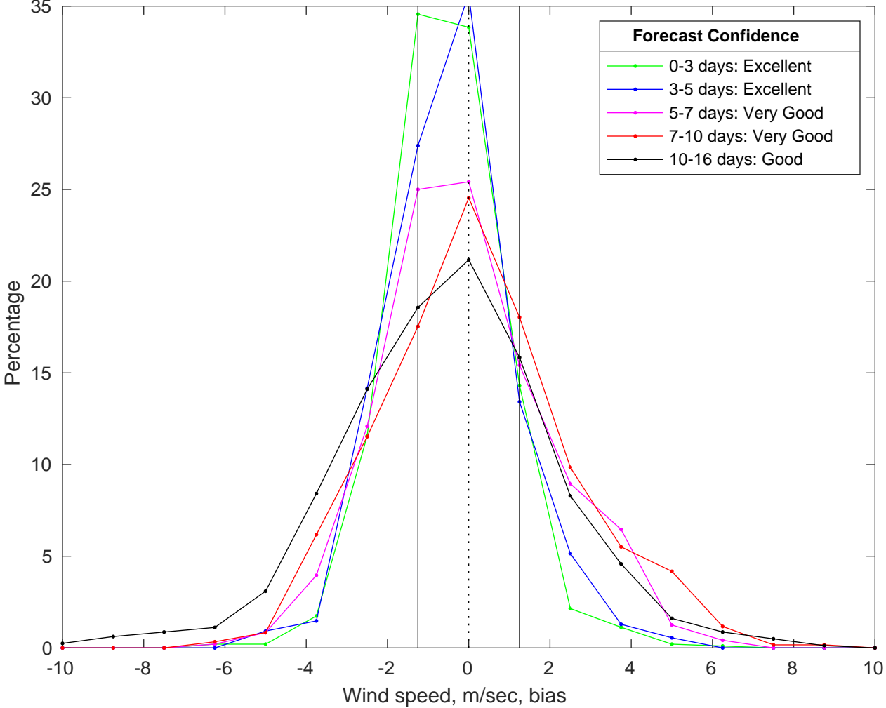
NDBC 41004 vs GFS Winds Bias Histogram: 03-Jul-2025
