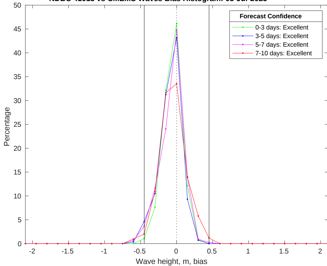
NDBC 41013 vs CMEMS Waves Bias Histogram: 03-Jul-2025
