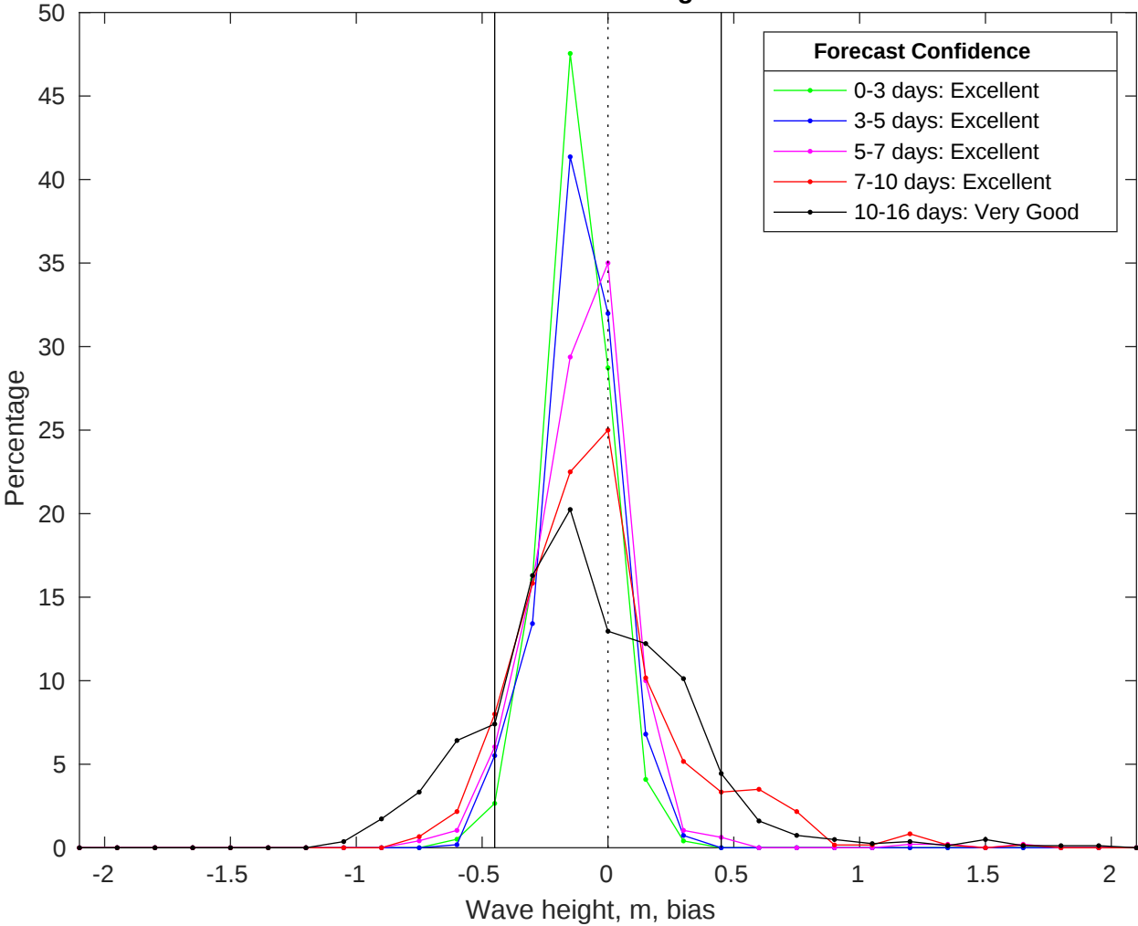
NDBC 41013 vs GFS Waves Bias Histogram: 03-Jul-2025
