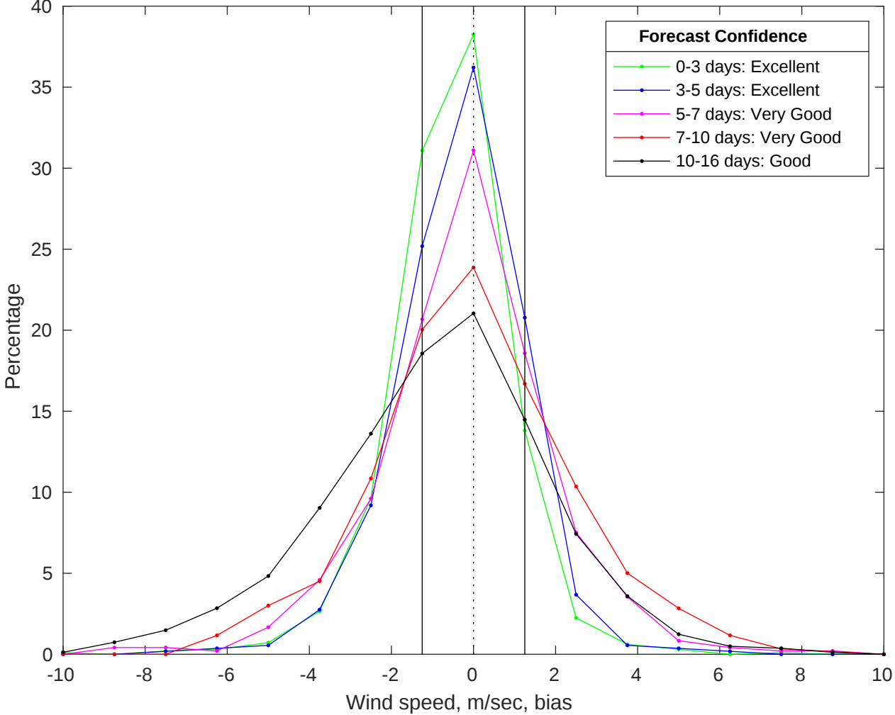
NDBC 41013 vs GFS Winds Bias Histogram: 03-Jul-2025
