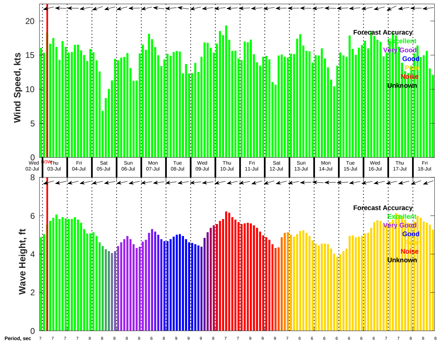
Wind & Wave Forecast for NDBC 41040 from 02-Jul-2025 21:00:00 to 18-Jul-2025 21:00:00
