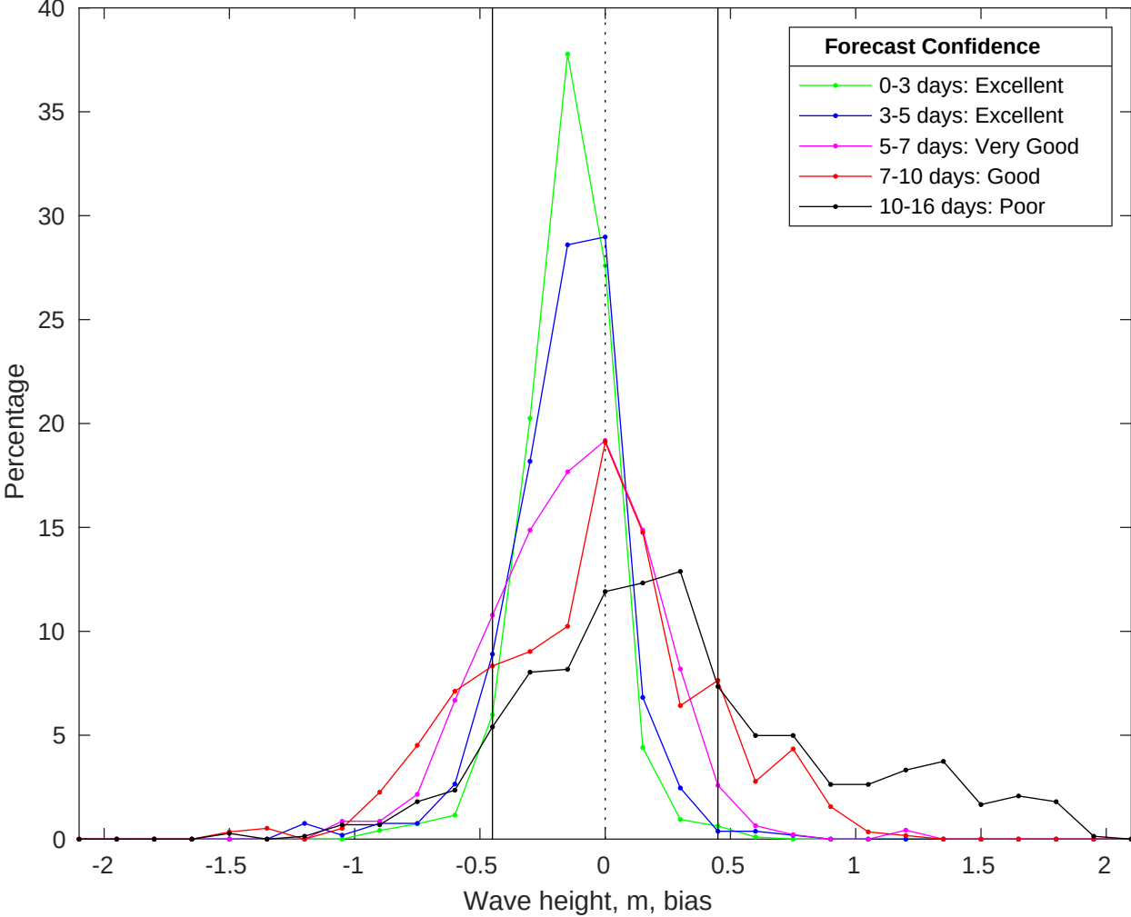
NDBC 42019 vs GFS Waves Bias Histogram: 03-Jul-2025
