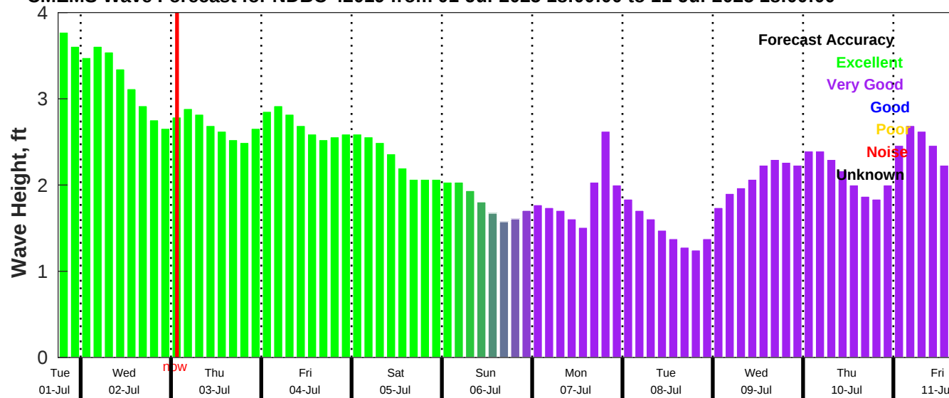
CMEMS Wave Forecast for NDBC 42019 from 01-Jul-2025 18:00:00 to 11-Jul-2025 18:00:00
