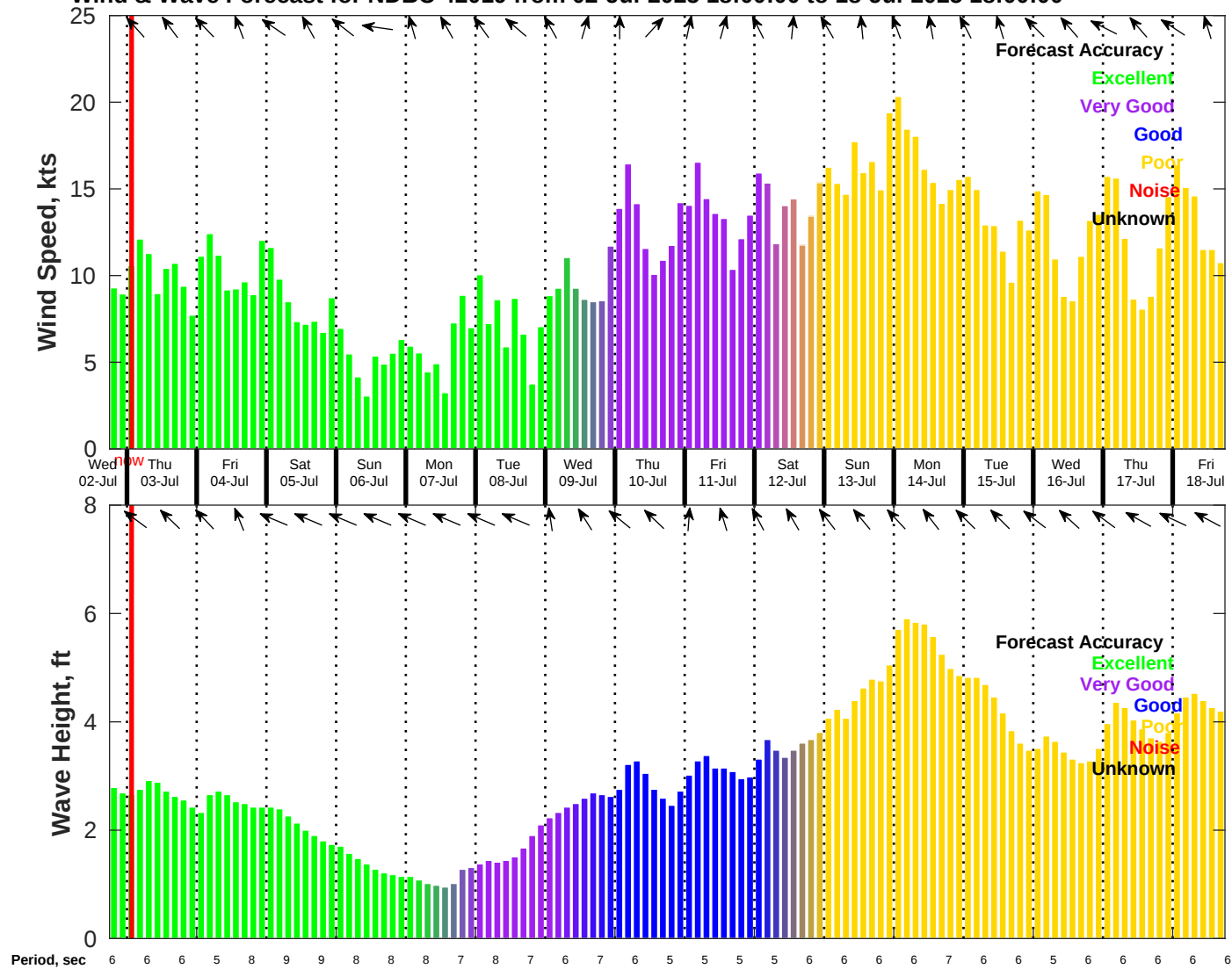
Wind & Wave Forecast for NDBC 42019 from 02-Jul-2025 18:00:00 to 18-Jul-2025 18:00:00
