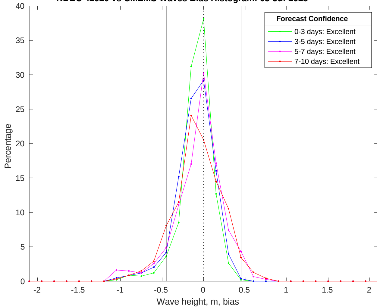
NDBC 42020 vs CMEMS Waves Bias Histogram: 03-Jul-2025
