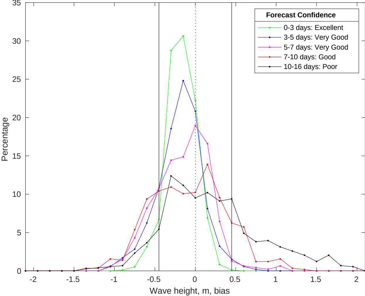
NDBC 42020 vs GFS Waves Bias Histogram: 03-Jul-2025
