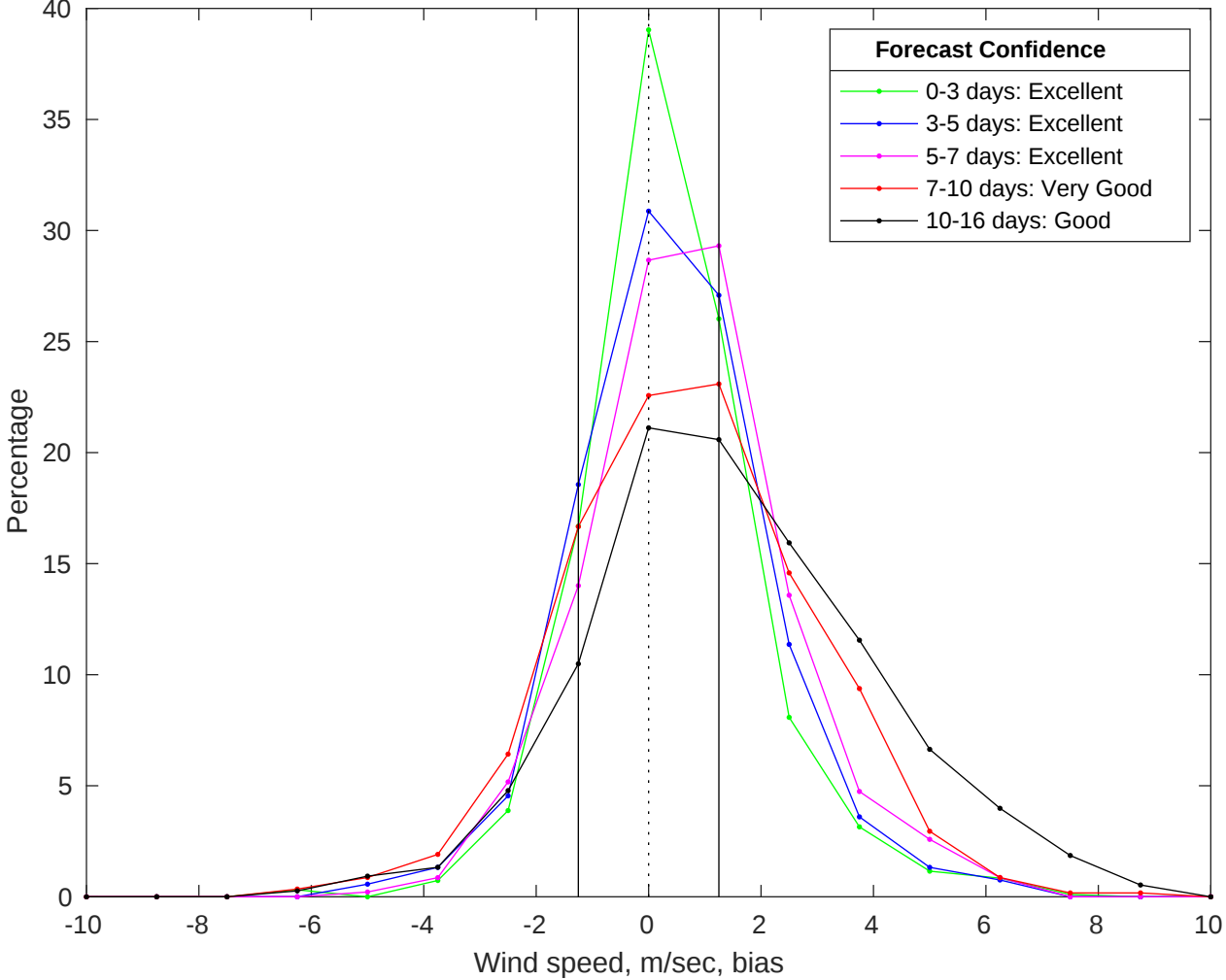
NDBC 42020 vs GFS Winds Bias Histogram: 03-Jul-2025
